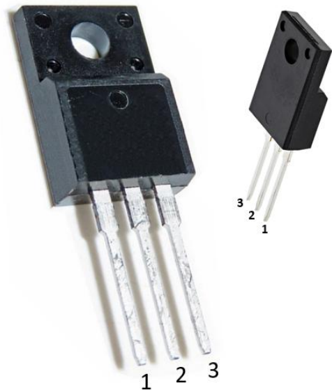
GR-65P240XF (TO-220-FP)
