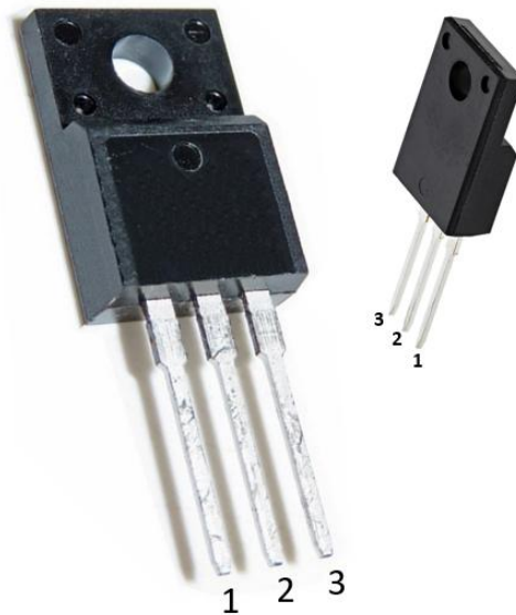
GR-65P100XF (TO-220-FP)
