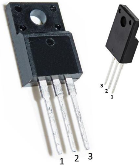
GR-65P075XF (TO-220-FP)
