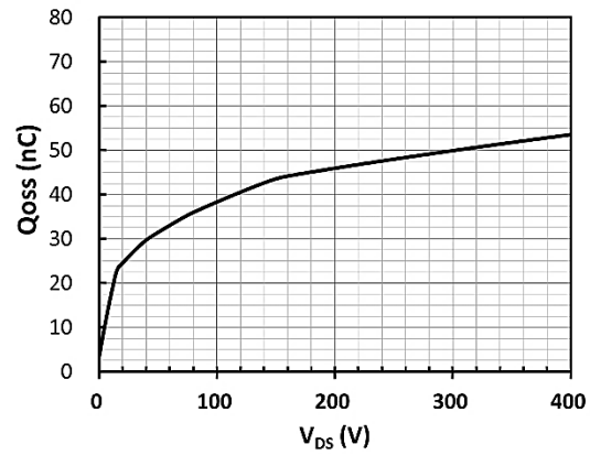
Fig 8. Capacitance Characteristics, Q_{oss}
