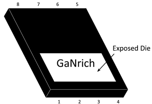
GR-20E010DJ, RQFN-5x6-8L
