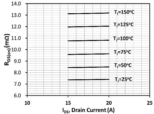
Fig 2. On-Resistance vs Drain Current and Temperature
