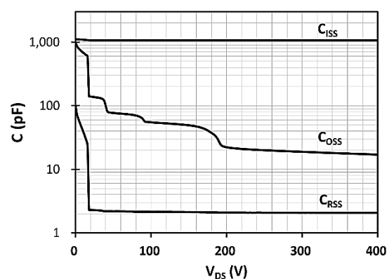
Fig 6. Capacitance Characteristics
