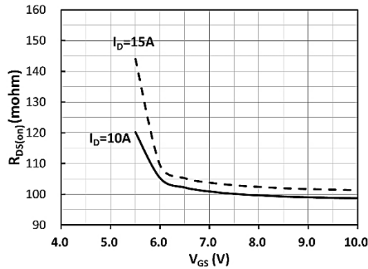
Fig 3. On-Resistance with Drain Current
