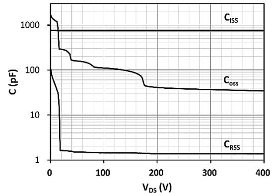
Fig 6. Capacitance Characteristics
