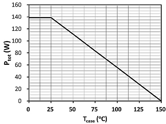
Fig 9. Power Dissipation Derating, P_{tot}
