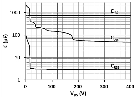
Fig 6. Capacitance Characteristics
