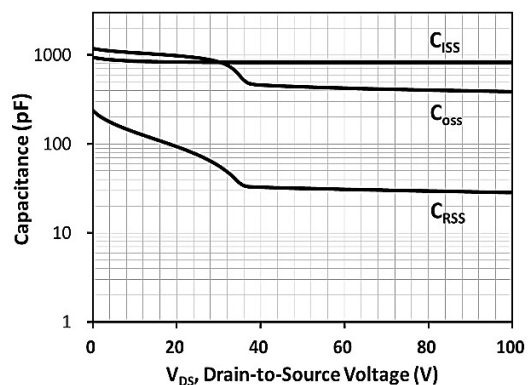
Fig 6. Capacitance Characteristics
