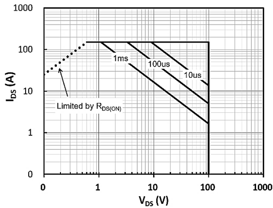
Fig 7. Safety Operation Area
